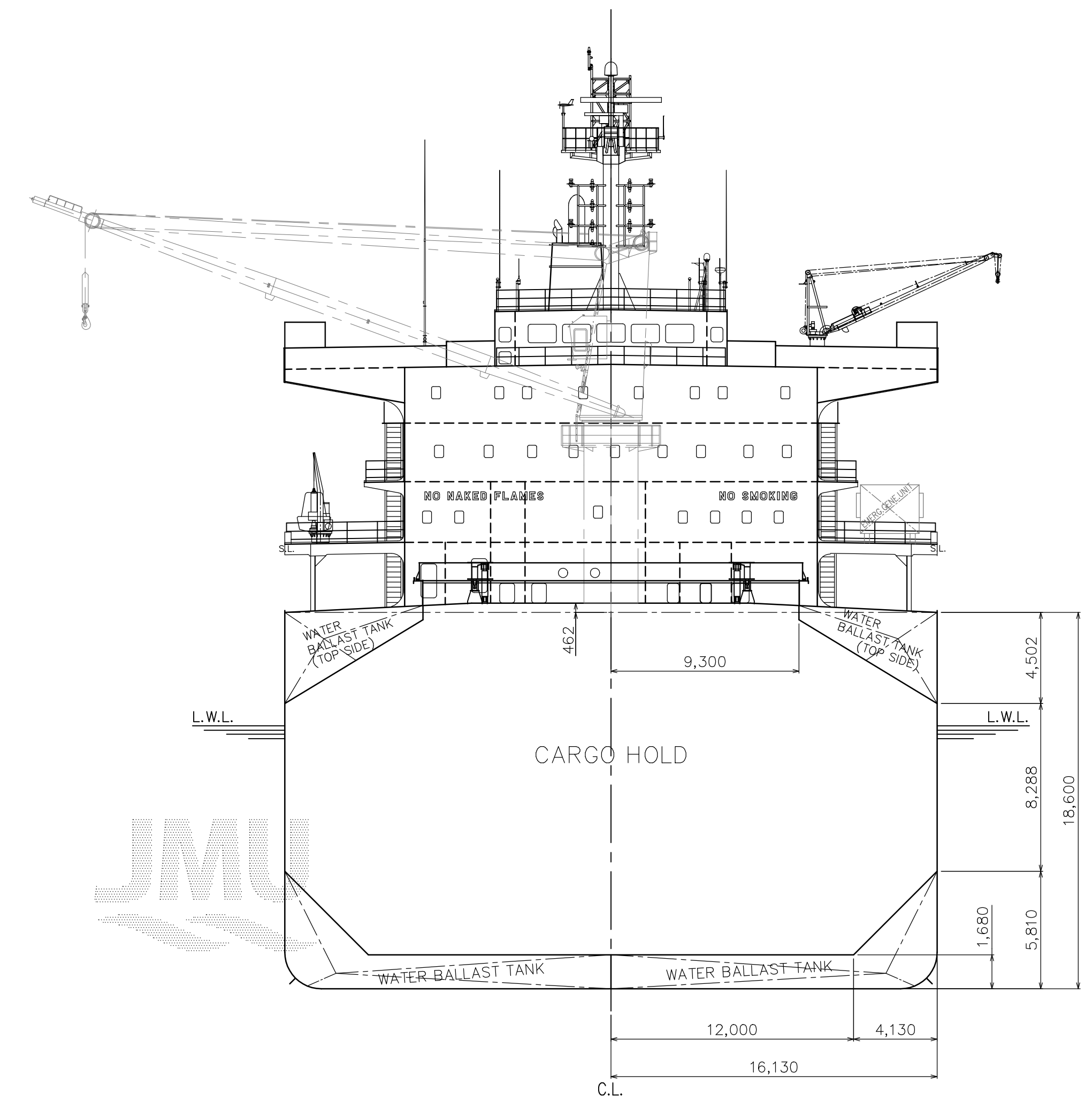
FRONT VIEW & MIDSHIP SECTION
